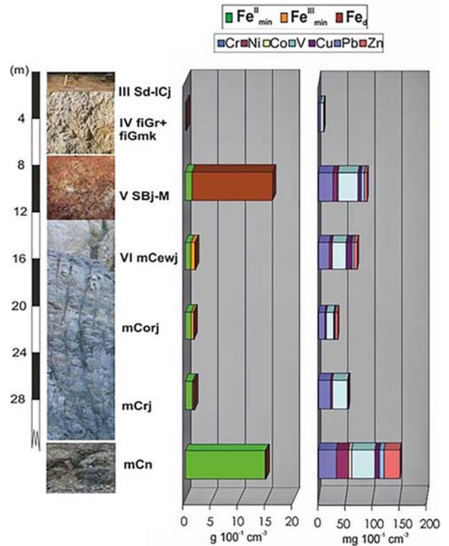
Figure 17. Eisenbach Öлкаute, semi-terrestrial saprolite: volumetric masses of iron fractions (mineralogically bound \text{Fe}^{\text{III}}_{\text{min}} and \text{Fe}^{\text{II}}_{\text{min}} , as well as free iron oxides \text{Fe}_D ) and trace elements of fresh slate and saprolite.
