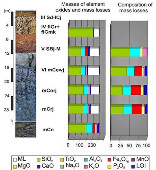
Figure 14. Eisenbach Ölkaut, semi-terrestrial saprolite: main element composition (vol-wt in \text{g } 100^{-1} \text{ cm}^{-3} ) of fresh slate and saprolite, isovolumetric bulk mass losses (ML) and relative elemental composition of mass losses (in % of the bulk mass loss).
