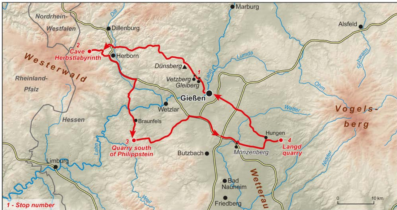
Figure 1. Topographic map with excursion route and major locations. Stop 1: Gleiberg and Vetzberg volcanoes, Stop 2: Herbstlabyrinth limestone cave, Stop 3: quarry south of Philippstein, Stop 4: abandoned quarry east of Langd.
